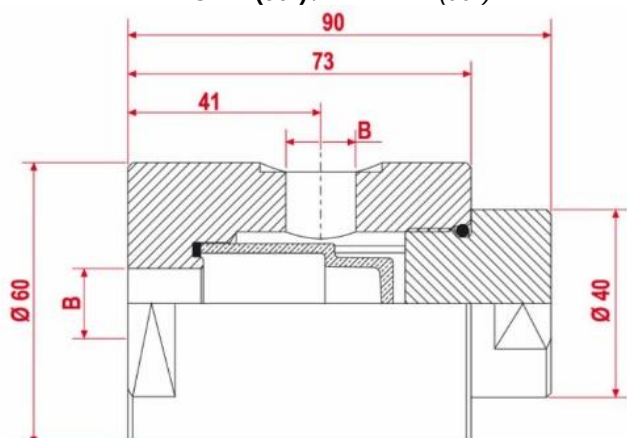
FILTRO A T(90°) / T-FILTER (90°)
