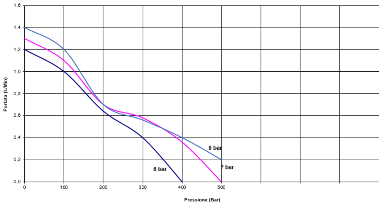
HP 500 - Oil Flow Diagram
