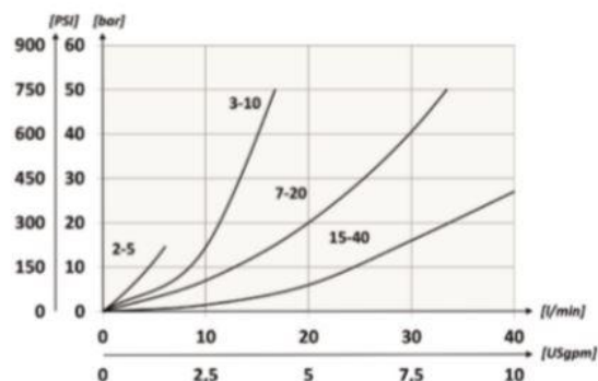
Rif. curva 2-5 relativa alla valvola VDRF101 Ref. to curve 2-5 for the VDRF101 valve
