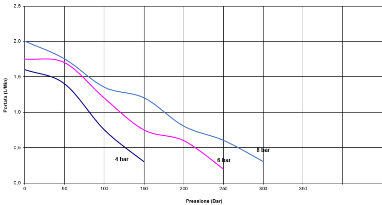
HP 250 - Oil Flow Diagram
